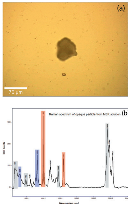
Figure 8: (a) Confocal Raman microscope image of opaque or white particle from MEK-diluted intermediate solution selected for Raman analysis; (b) Raman spectrum of particle in (a) suggests a mixture of fluoropolymer (blue), residual intermediate product or monomer (grey), and polystyrene (orange). Refer to Table I for color codes of monomer and raw materials.
