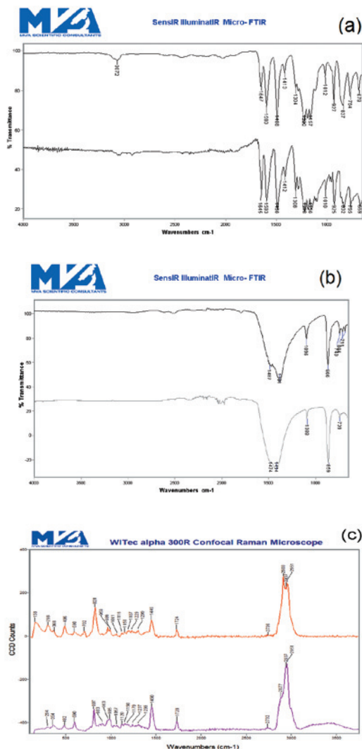
Figure 7: (a) Infrared spectrum (upper trace) of particle identified as extraneous material isolated from haziest monomer solution and polyether ether ketone (PEEK) reference (lower trace); (b) infrared spectrum (upper trace) of particle identified as extraneous material isolated from haziest monomer solution and inorganic carbonate reference (lower trace); (c) Raman spectrum (upper trace) of opaque or white particle identified as extraneous material isolated from haziest monomer solution and CarboSet acrylic reference (lower trace).
