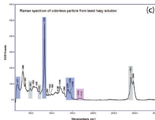
Figure 4: (a) Representative image of bumpy, textured particle selected for Raman analysis; (b) Raman spectrum of particle in (a), primarily fluoropolymer (blue) and monomer (grey); (c) Raman spectrum from additional clear or colorless particle showing a mixture of fluoropolymer (blue) and monomer (grey) with traces of isocyanate (pink). Refer to Table I for peak color codes of monomer and raw materials.
