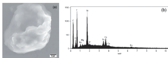
Figure 3: (a) SEM image of bumpy, textured particle isolated from least hazy monomer solution; (b) EDS spectrum from particle shown in (a).
