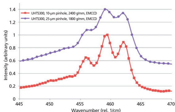
Figure 2: Raman spectrum of \text{CCl}_4 with 532-nm excitation at different spectral resolutions.
