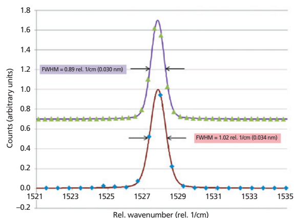
Figure 1: Spectra of the mercury atomic emission line at 579.066 nm plotted as a function of wavenumber assuming a 532.00-nm excitation. The red line is the fitted curve (pseudo voight function) and the blue diamonds are the measured data points for the 1800-grooves/mm grating. The green triangles and the purple curve show the results obtained using the 2400-grooves/mm grating.
